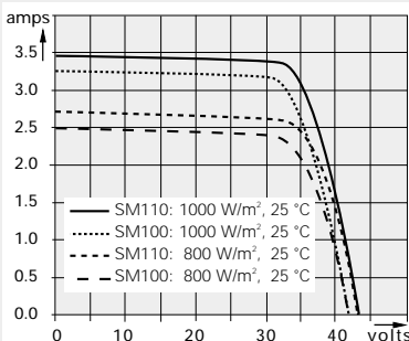
Voltage-current characteristic 24 V
